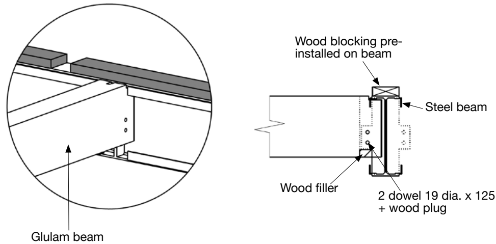
Glulam to steel I-beam connection
