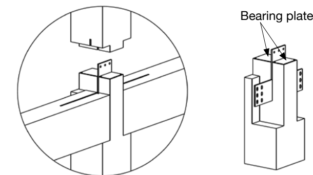
Typical hole in column bearing plate
