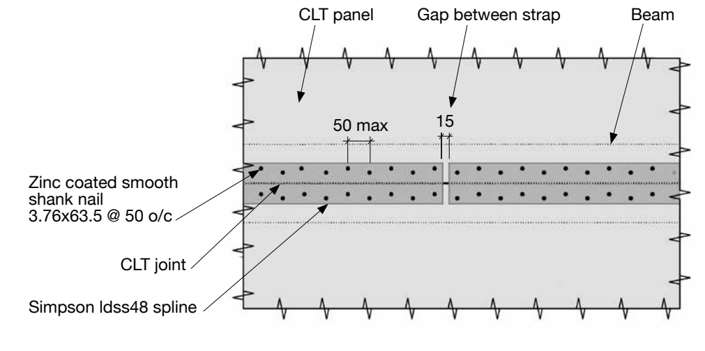
Plan - CLT to CLT joint with spline
