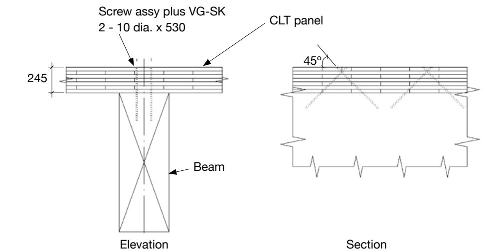
Screwing pattern CLT panel to beam
